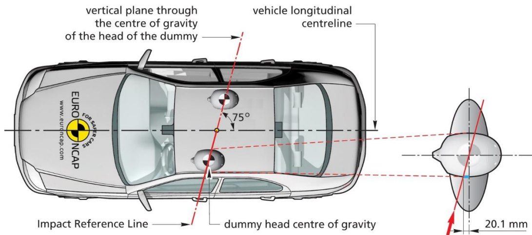
Figure 2: Pole impact reference line (IRL)
