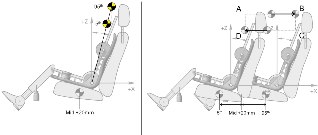
Figure 7: HPD zone front seat row
