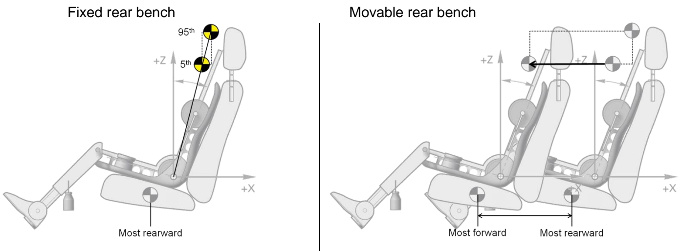
Figure 8: HPD zone rear seat row(s)
