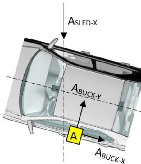
Figure 4: Far side impact
