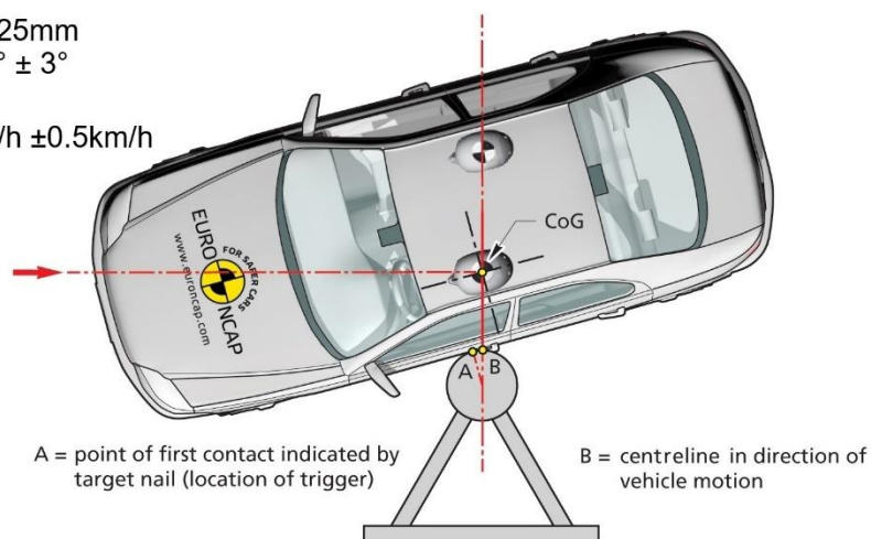
Figure 3: Pole impact location
