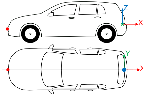
Figure 1 – Euro NCAP Vehicle Coordinate System
